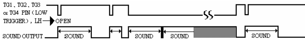
TRIGGER MODE : ONE SHOT RE-TRIGGER
